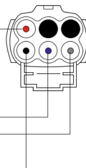
6 pins Sumitomo male connector pinout contact insertion view
