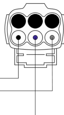
6 pins Sumitomo male connector pinout contact insertion view
