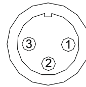
3 pins Binder 712 male connector pinout solder termination view
