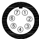
7 pins Binder 12 male connector pinout solder termination view
